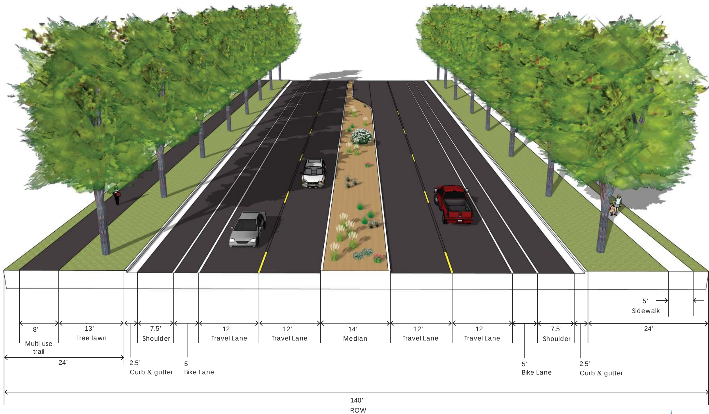
REDWOOD ROAD STREET SECTION
